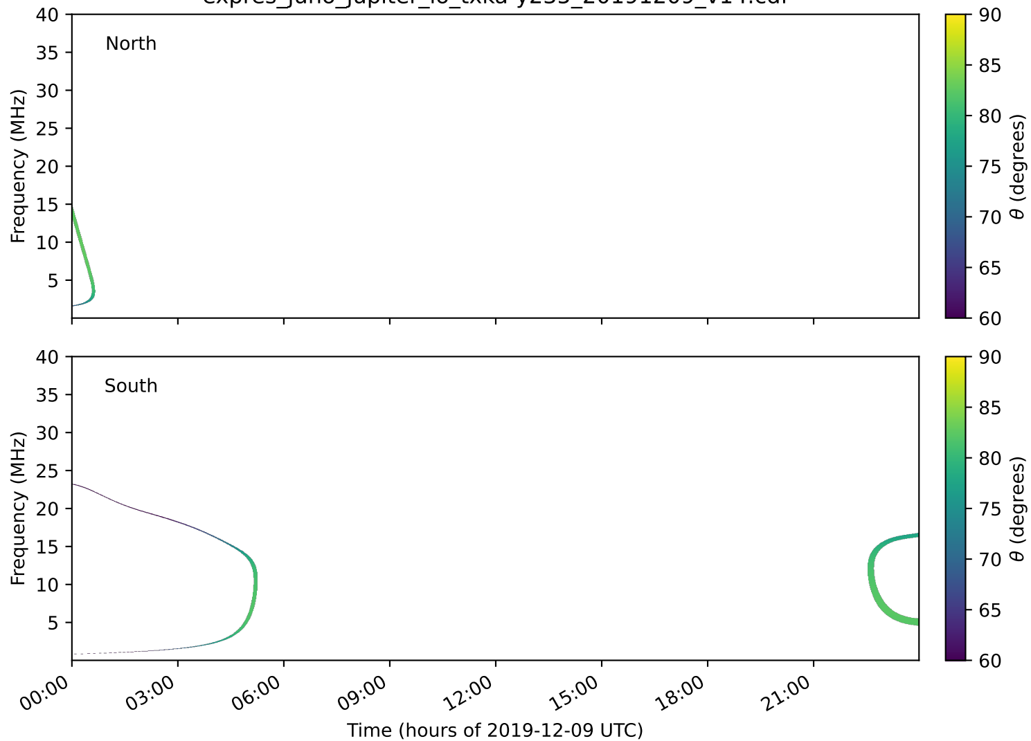
expres_juno_jupiter_io_txka-y235_20191209_v14.cdf
