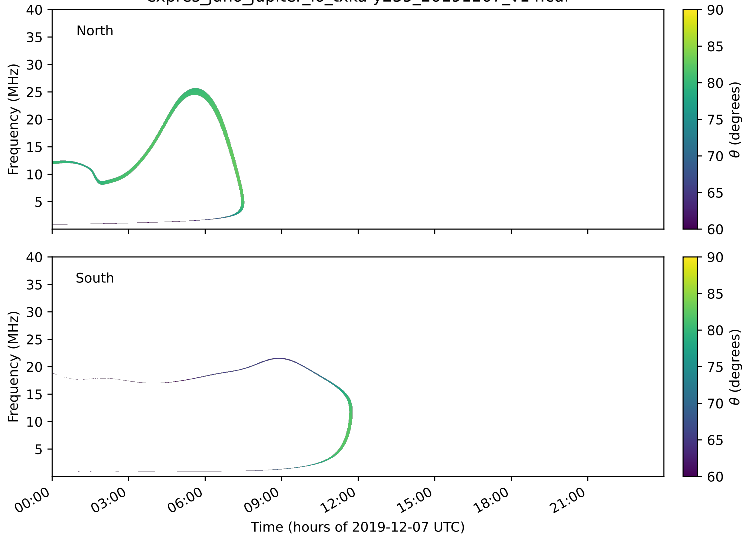
expres_juno_jupiter_io_txka-y235_20191207_v14.cdf
