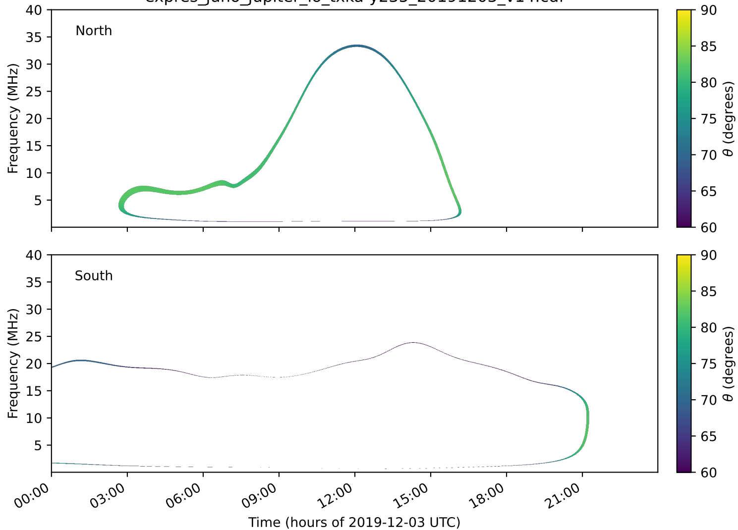
expres_juno_jupiter_io_txka-y235_20191203_v14.cdf
