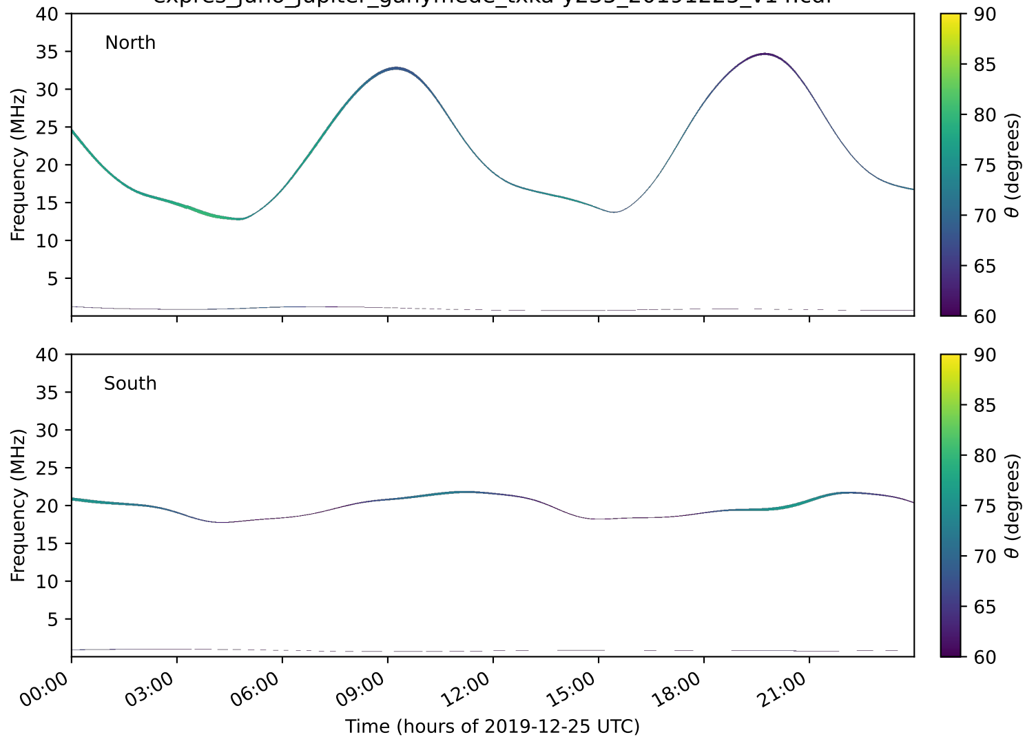
expres_juno_jupiter_ganymede_txka-y235_20191225_v14.cdf
