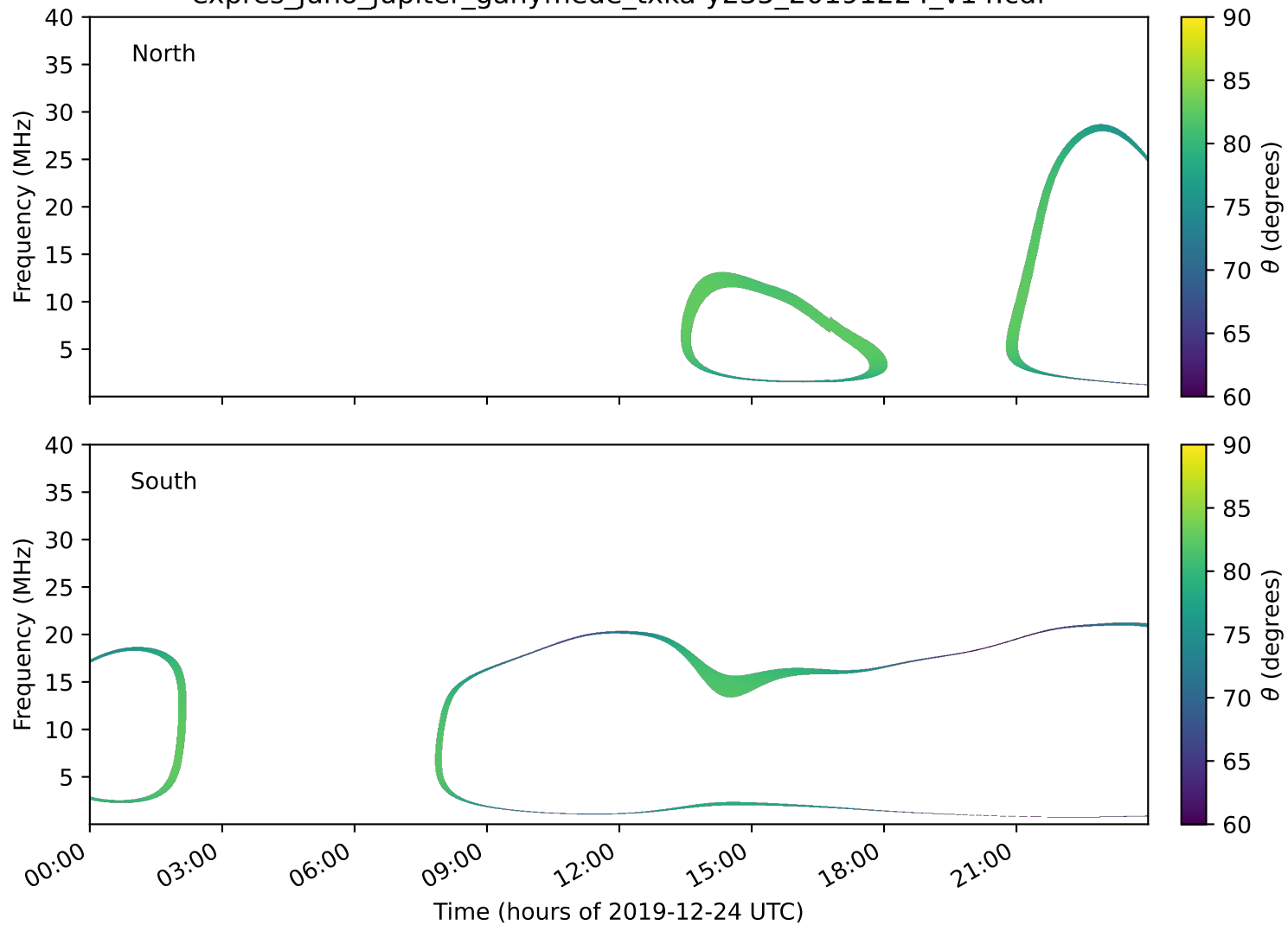
expres_juno_jupiter_ganymede_txka-y235_20191224_v14.cdf
