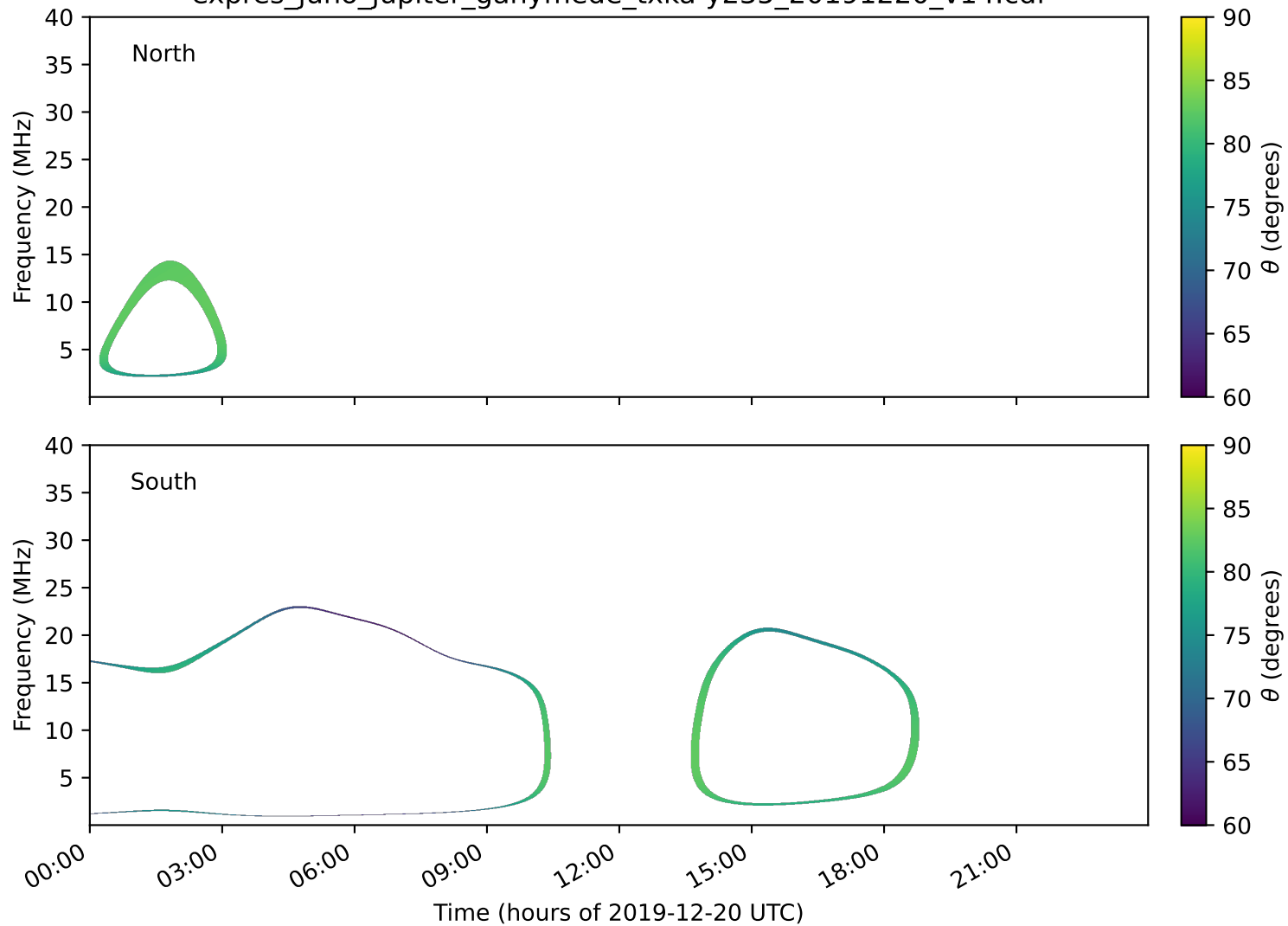
expres_juno_jupiter_ganymede_txka-y235_20191220_v14.cdf
