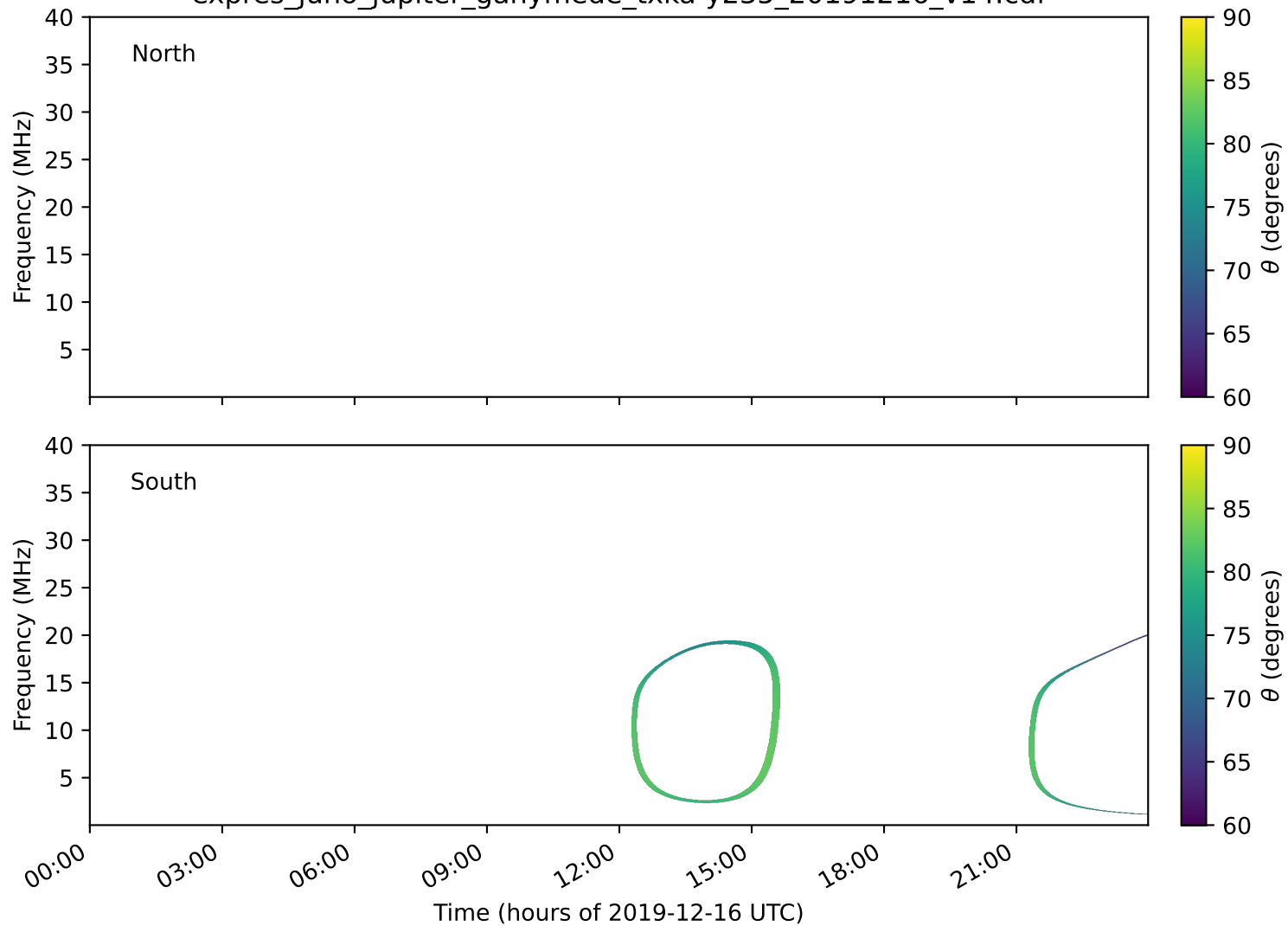
expres_juno_jupiter_ganymede_txka-y235_20191216_v14.cdf
