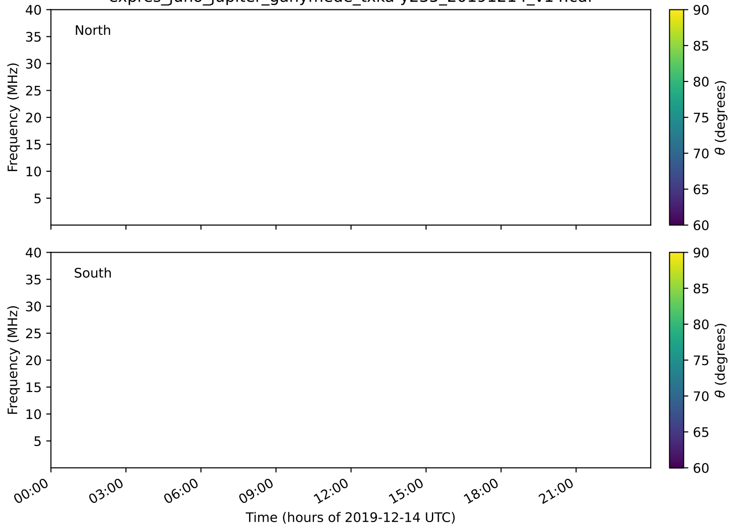
expres_juno_jupiter_ganymede_txka-y235_20191214_v14.cdf
