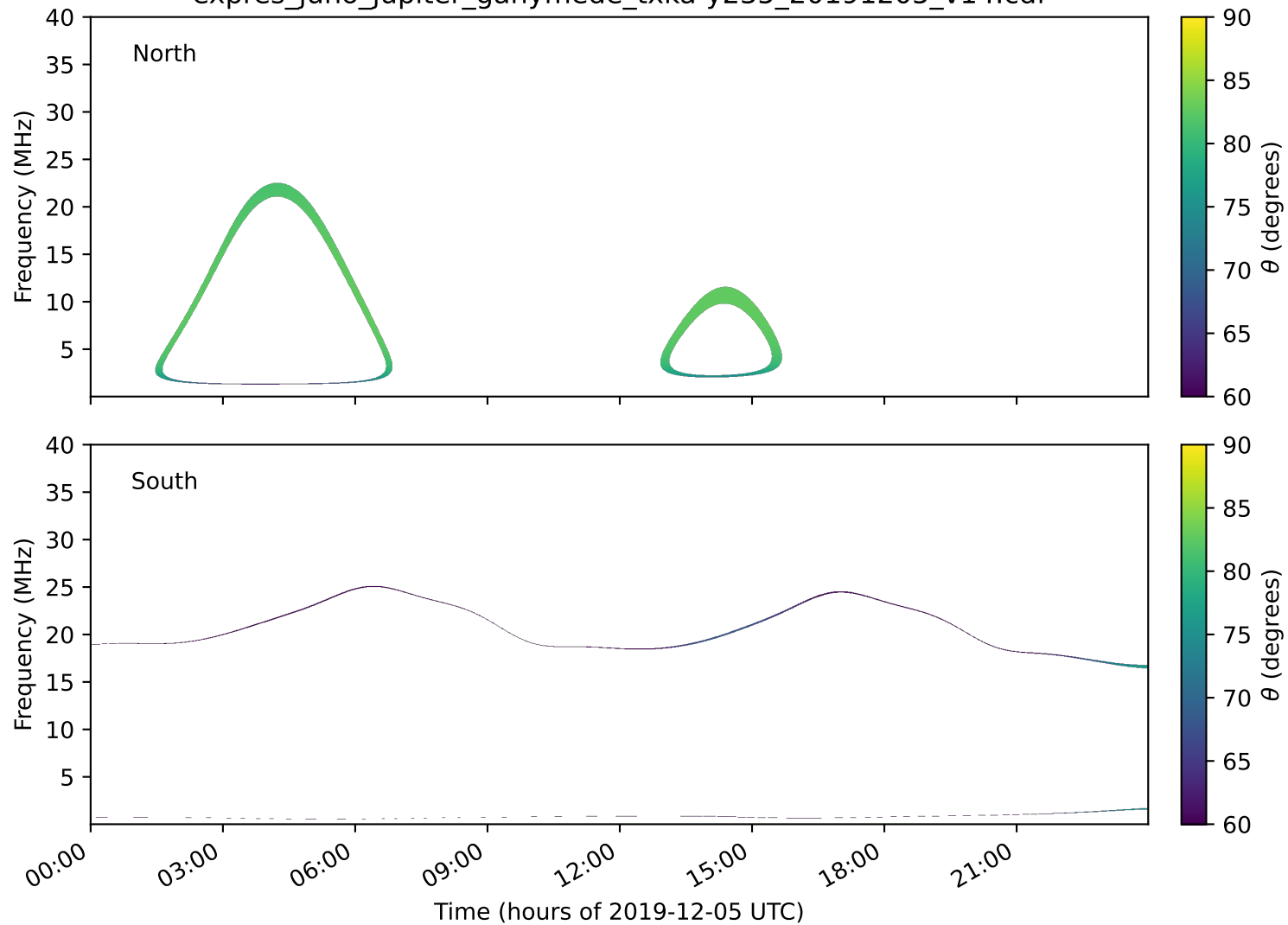
expres_juno_jupiter_ganymede_txka-y235_20191205_v14.cdf
