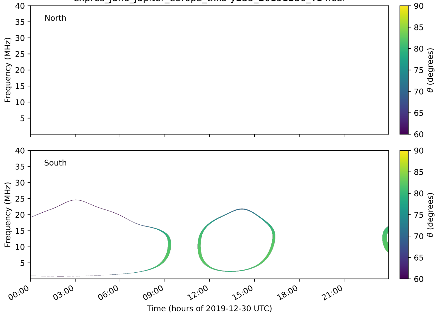
expres_juno_jupiter_europa_txka-y235_20191230_v14.cdf
