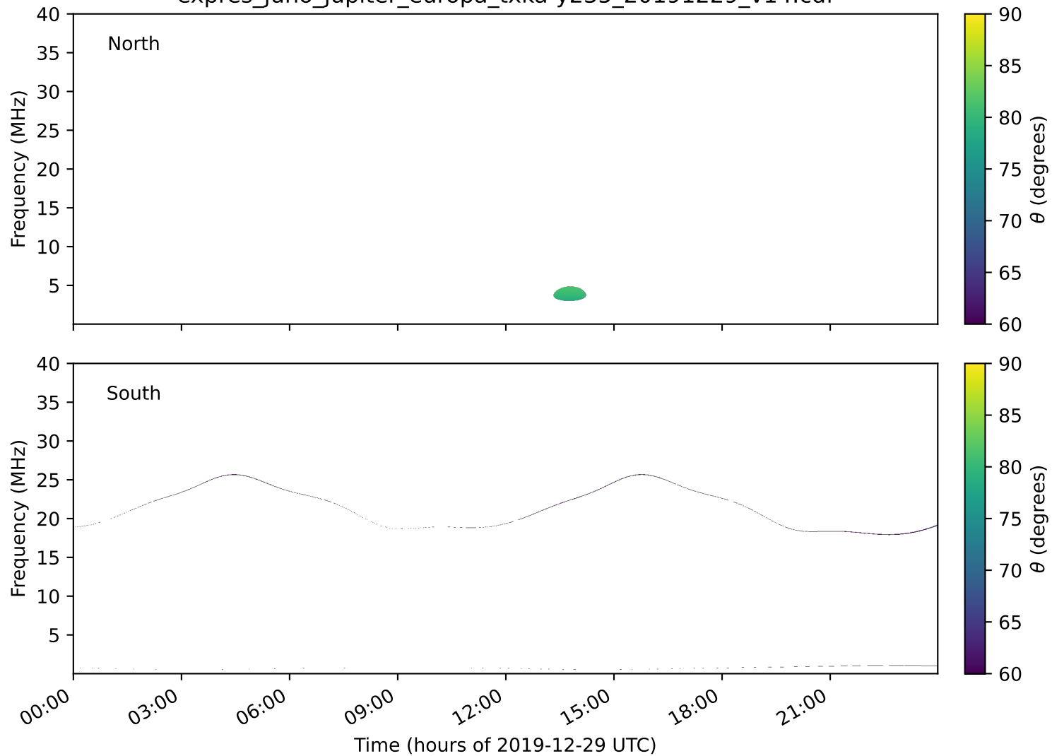
expres_juno_jupiter_europa_txka-y235_20191229_v14.cdf
