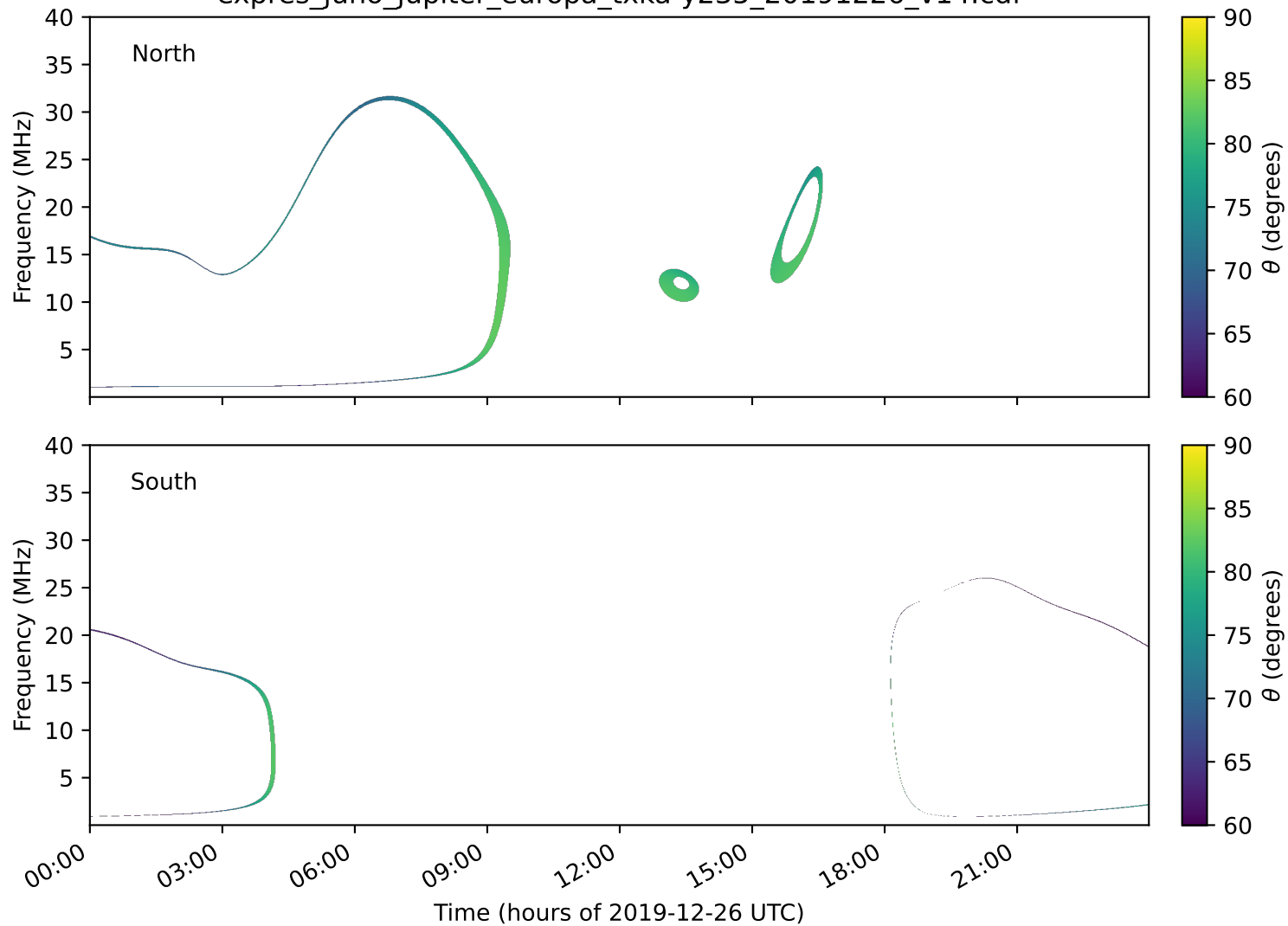
expres_juno_jupiter_europa_txka-y235_20191226_v14.cdf
