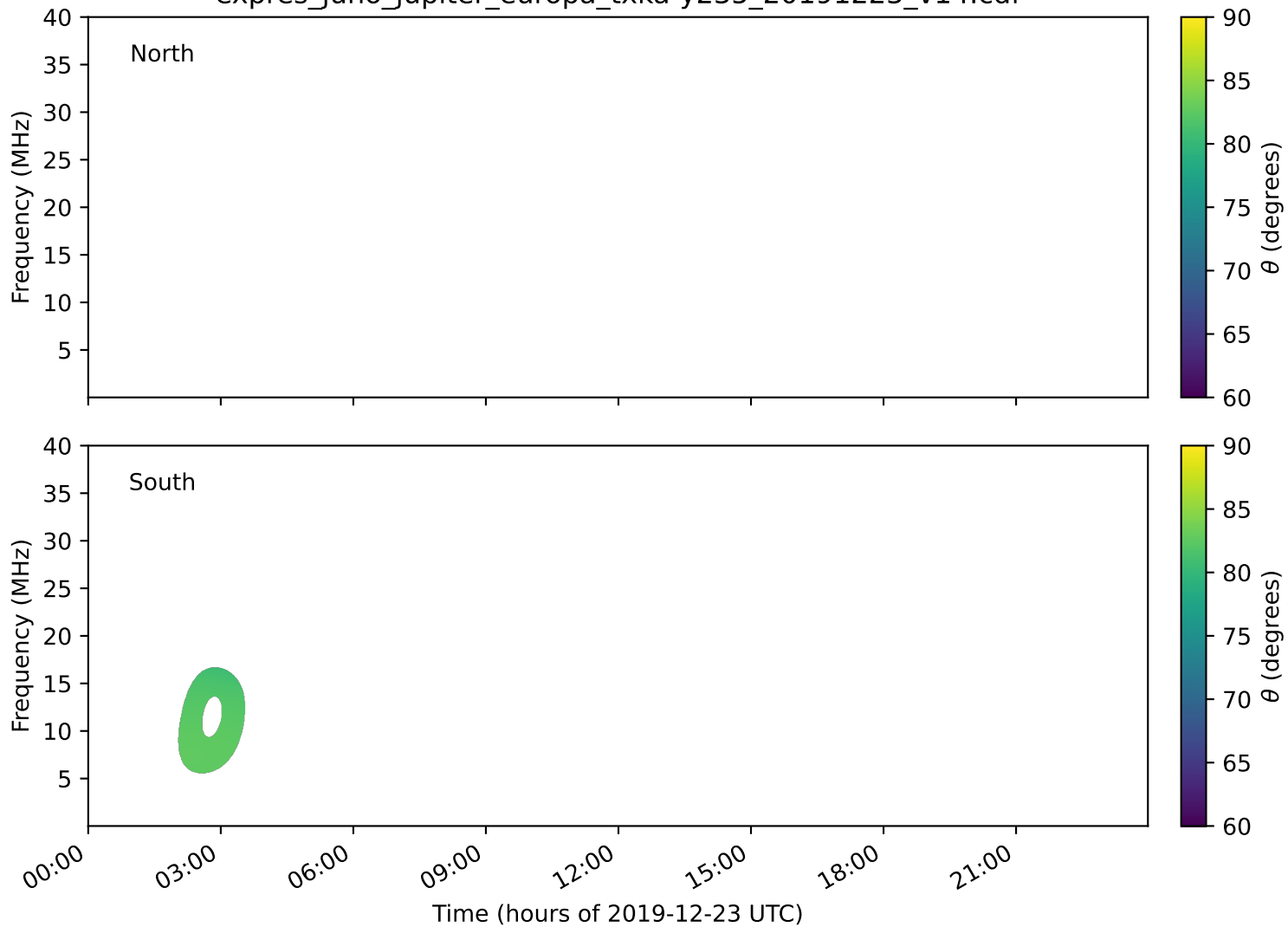
expres_juno_jupiter_europa_txka-y235_20191223_v14.cdf
