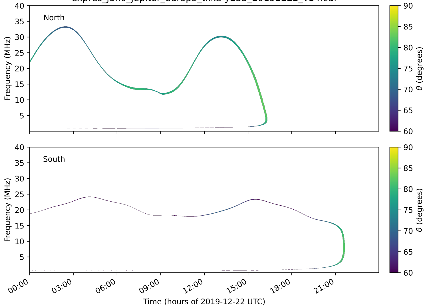
expres_juno_jupiter_europa_txka-y235_20191222_v14.cdf
