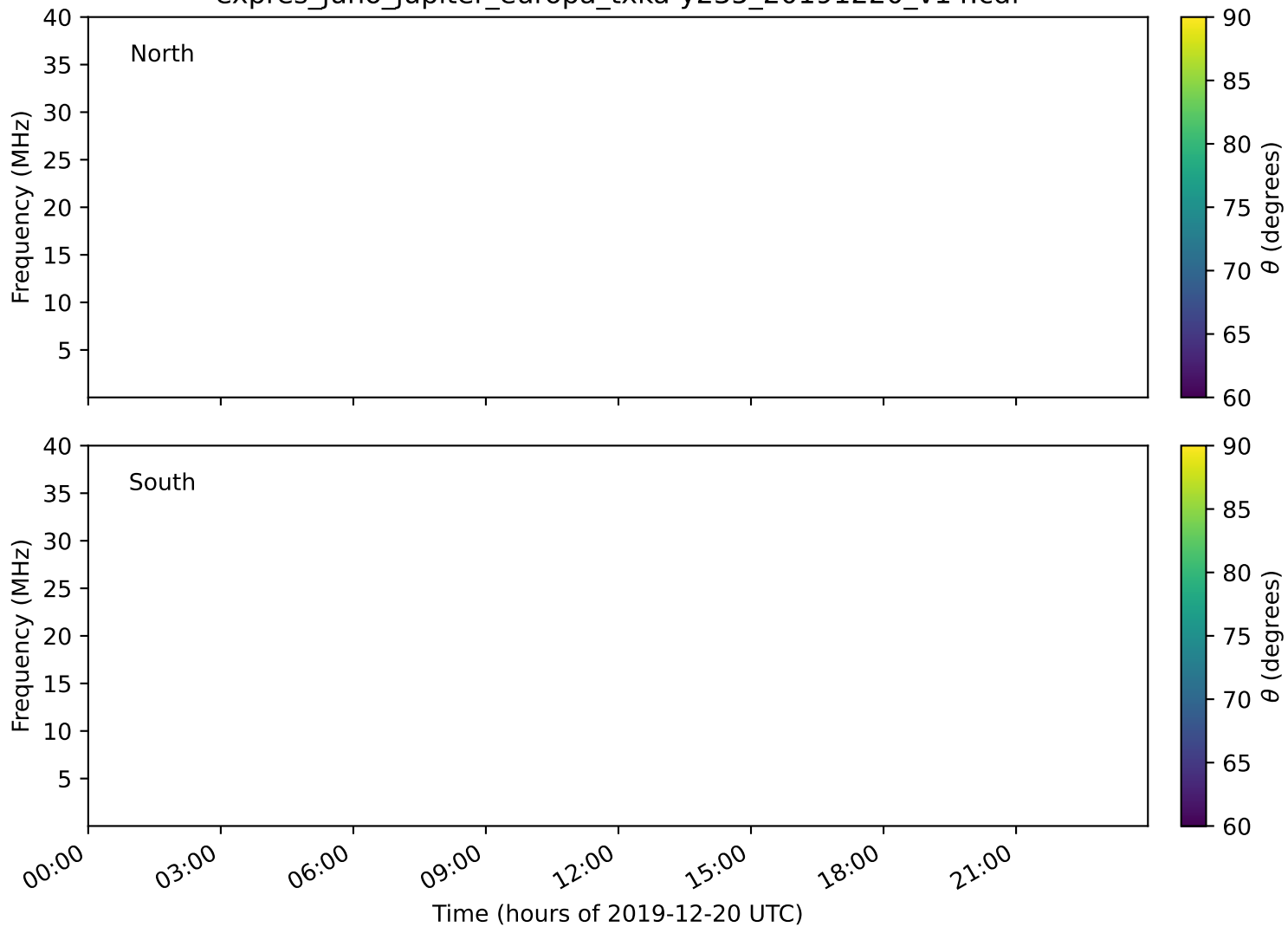
expres_juno_jupiter_europa_txka-y235_20191220_v14.cdf
