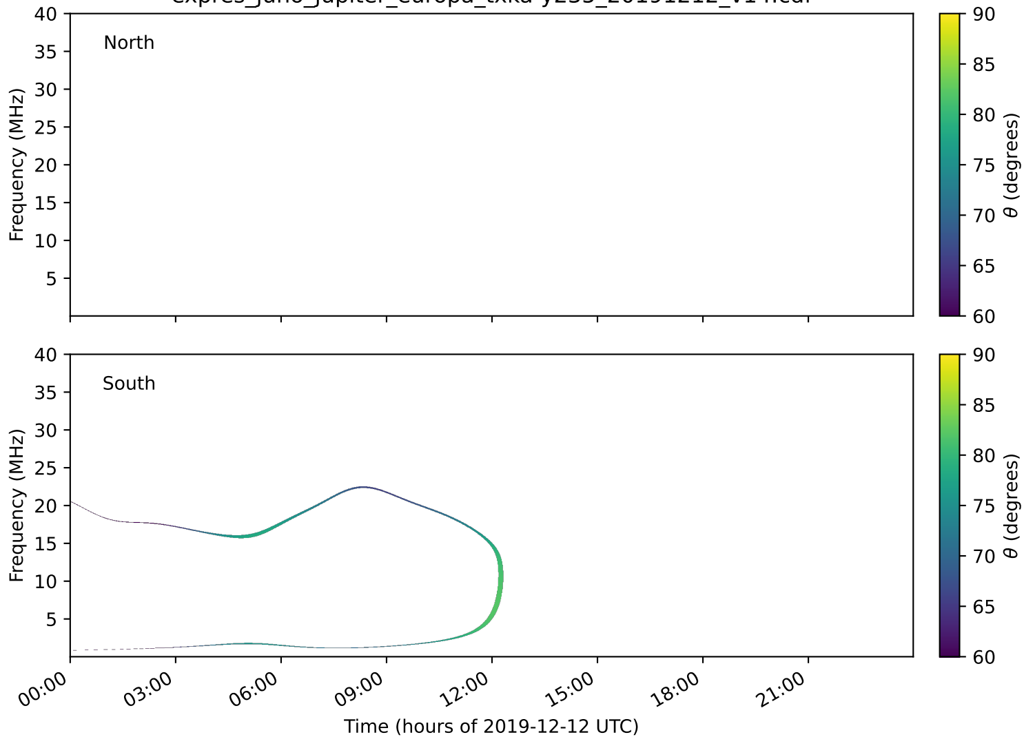
expres_juno_jupiter_europa_txka-y235_20191212_v14.cdf
