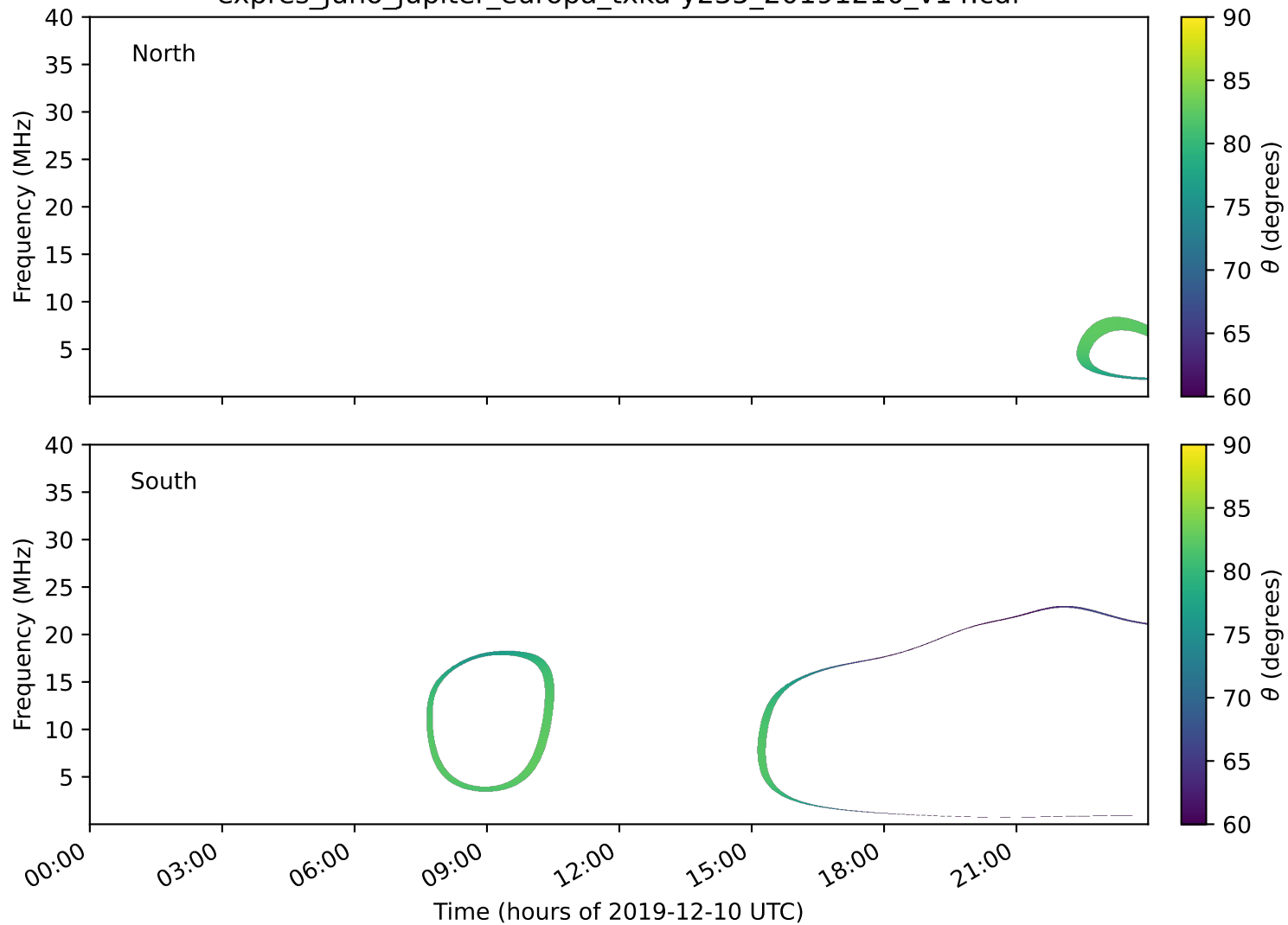
expres_juno_jupiter_europa_txka-y235_20191210_v14.cdf
