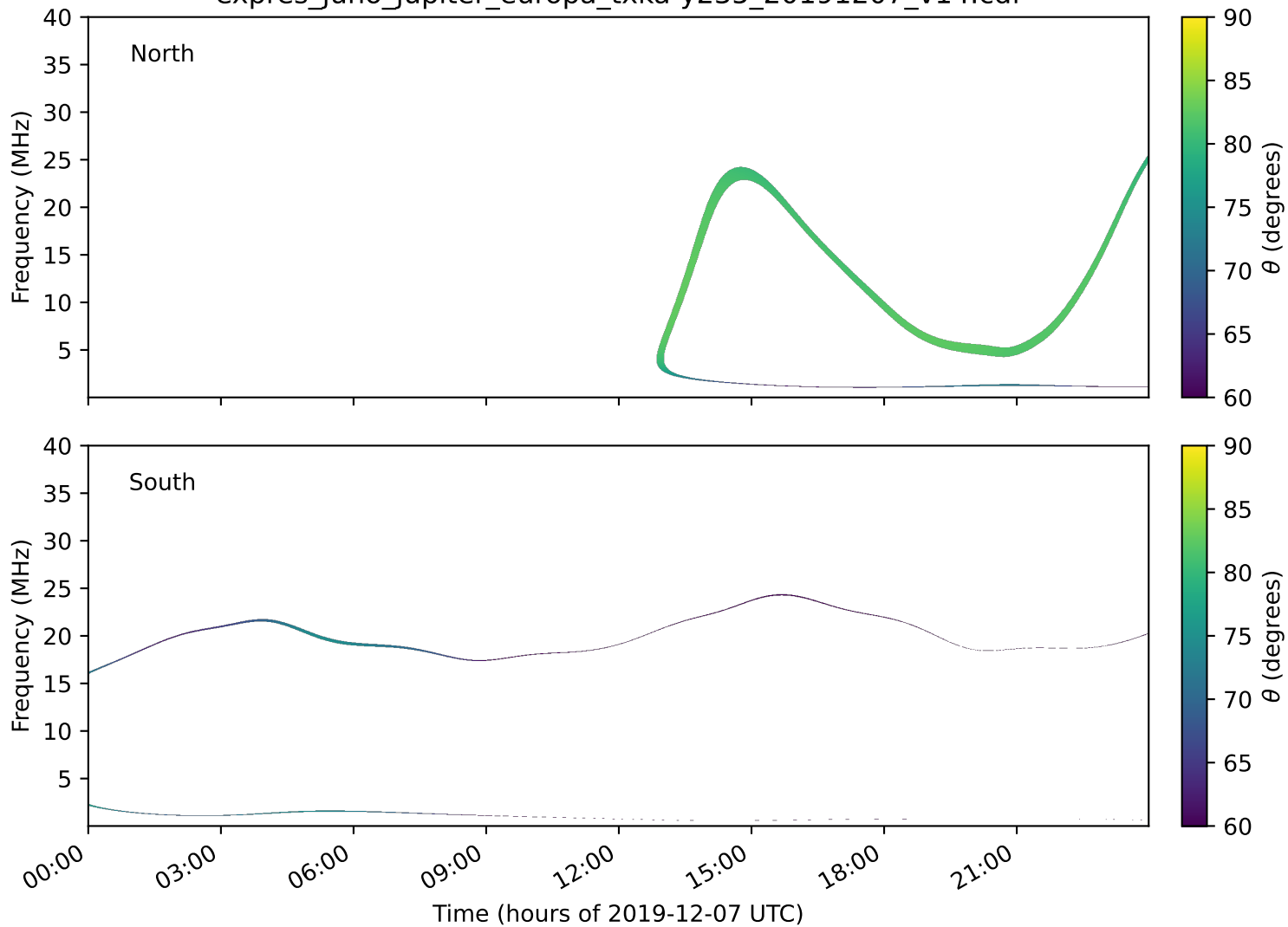
expres_juno_jupiter_europa_txka-y235_20191207_v14.cdf
