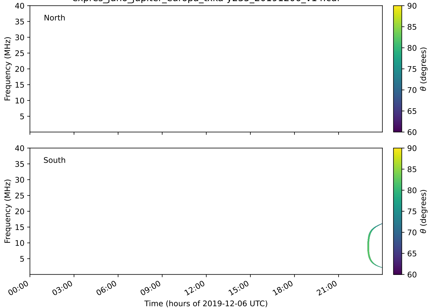
expres_juno_jupiter_europa_txka-y235_20191206_v14.cdf
