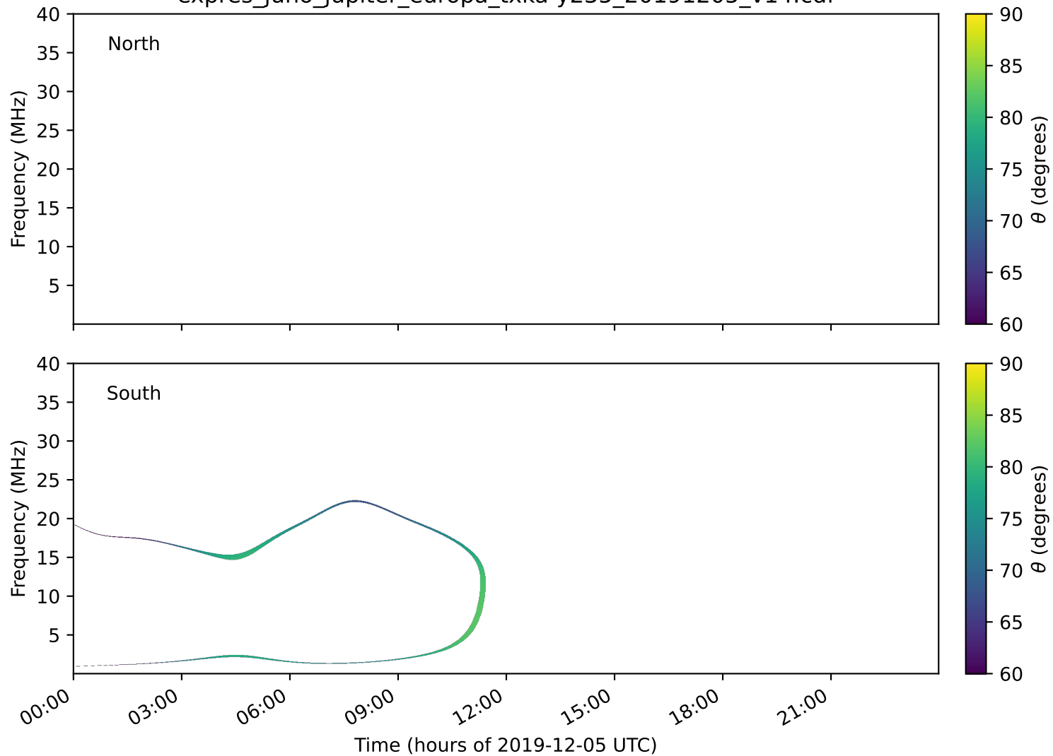
expres_juno_jupiter_europa_txka-y235_20191205_v14.cdf
