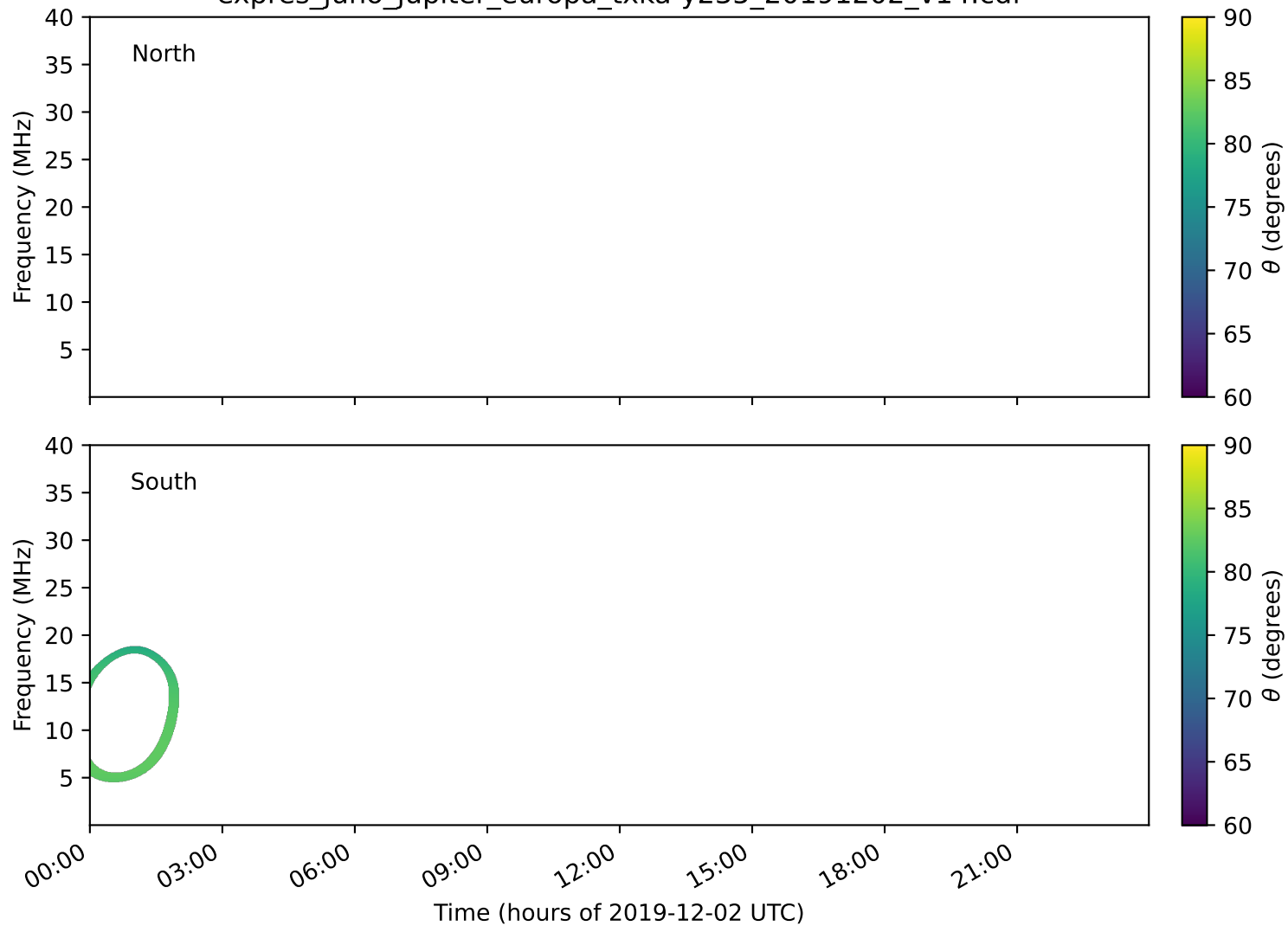
expres_juno_jupiter_europa_txka-y235_20191202_v14.cdf
