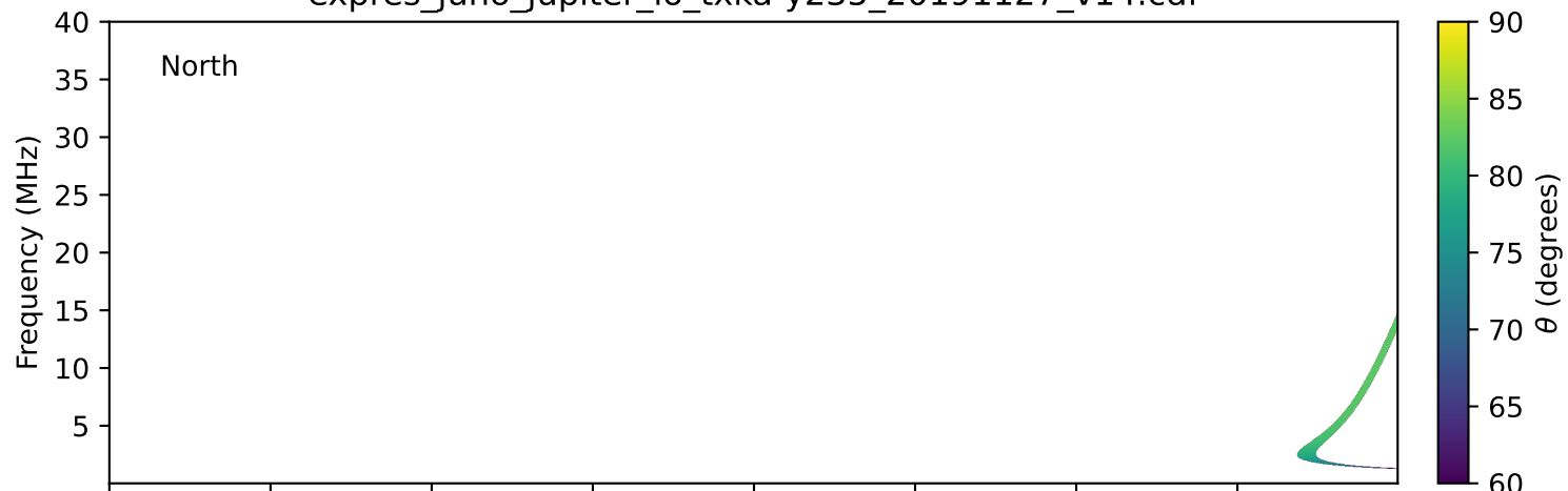
expres_juno_jupiter_io_txka-y235_20191127_v14.cdf
