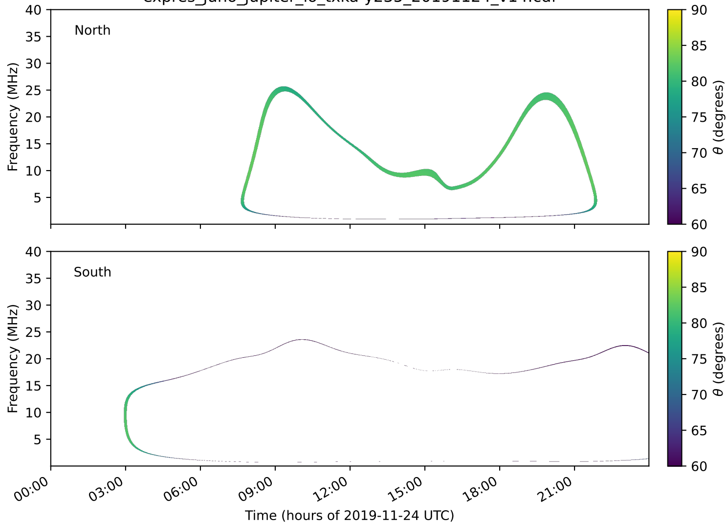
expres_juno_jupiter_io_txka-y235_20191124_v14.cdf
