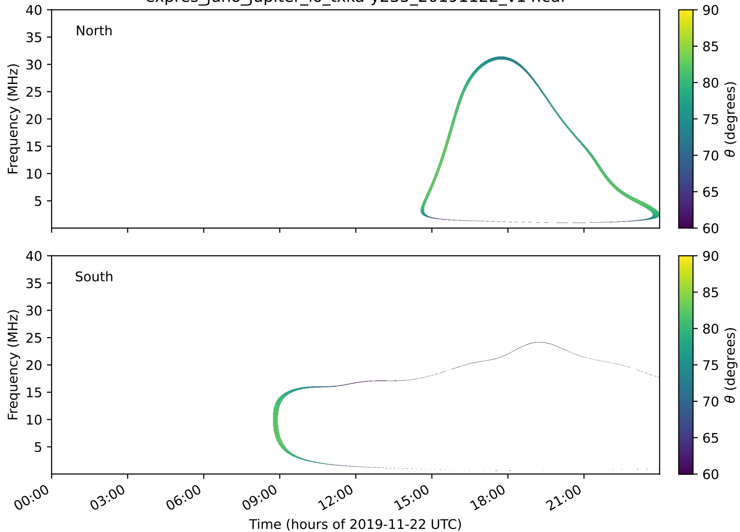
expres_juno_jupiter_io_txka-y235_20191122_v14.cdf
