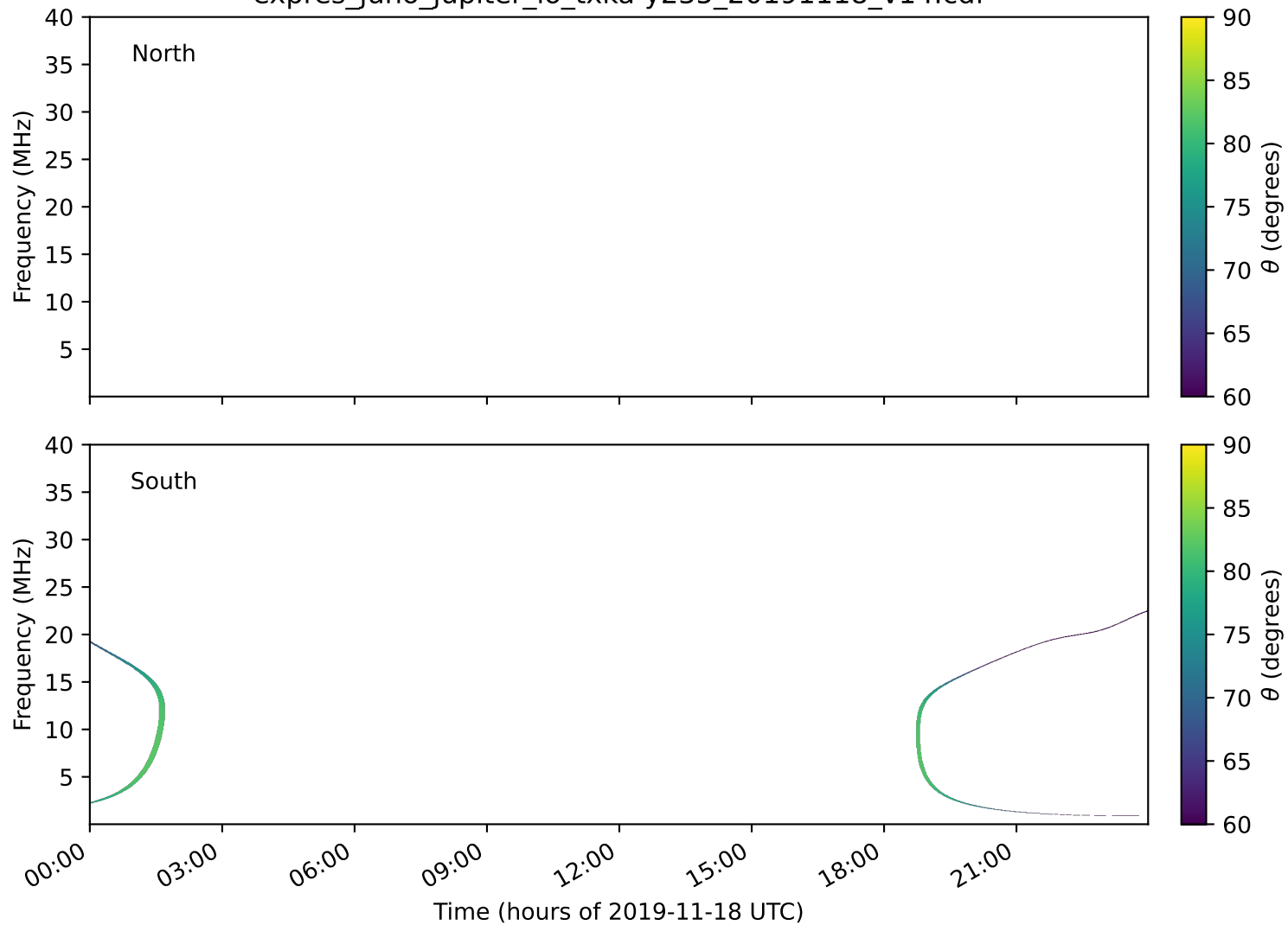
expres_juno_jupiter_io_txka-y235_20191118_v14.cdf
