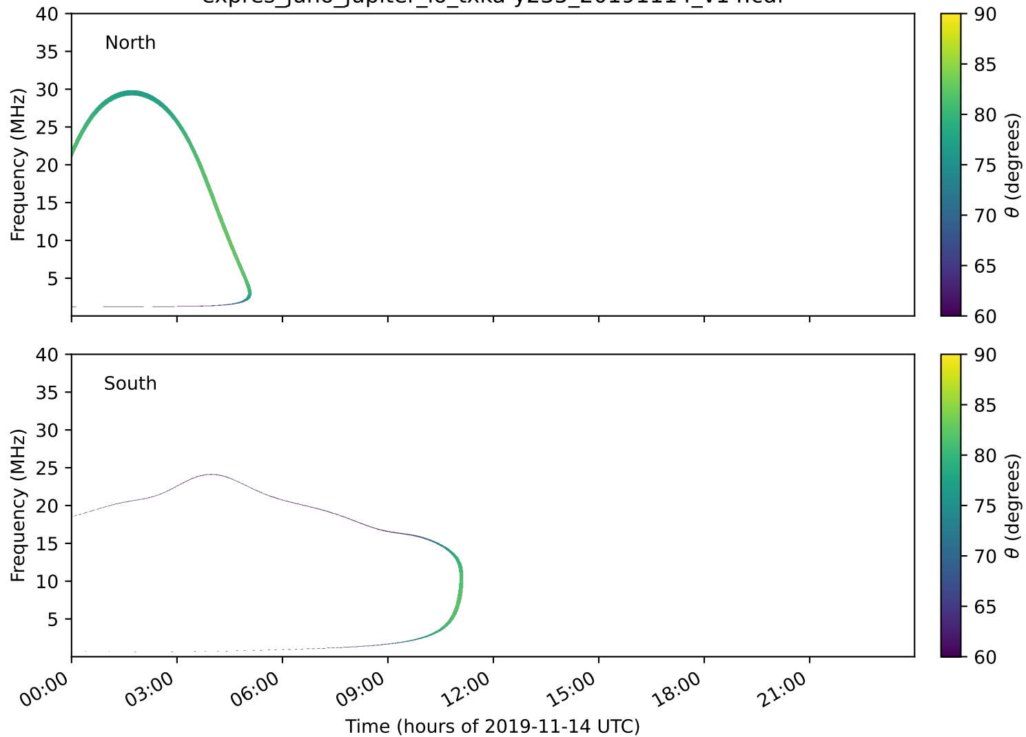
expres_juno_jupiter_io_txka-y235_20191114_v14.cdf
