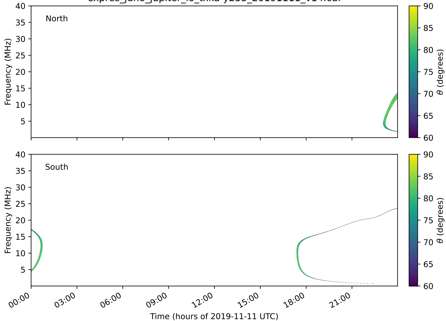
expres_juno_jupiter_io_txka-y235_20191111_v14.cdf
