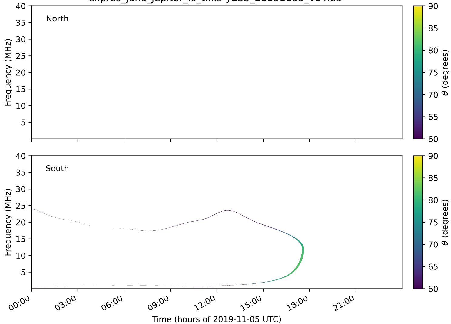
expres_juno_jupiter_io_txka-y235_20191105_v14.cdf
