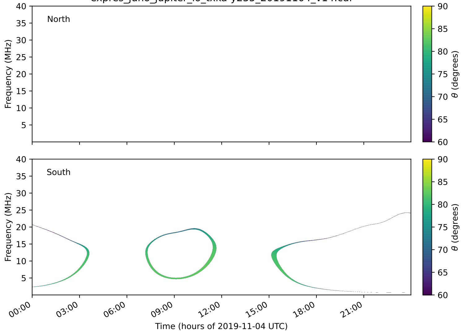
expres_juno_jupiter_io_txka-y235_20191104_v14.cdf
