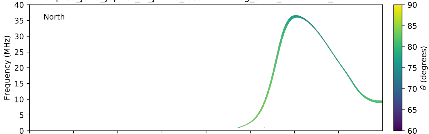
expres_juno_jupiter_io_jrm09_lossc-wid1deg_3kev_20191129_v01.cdf
