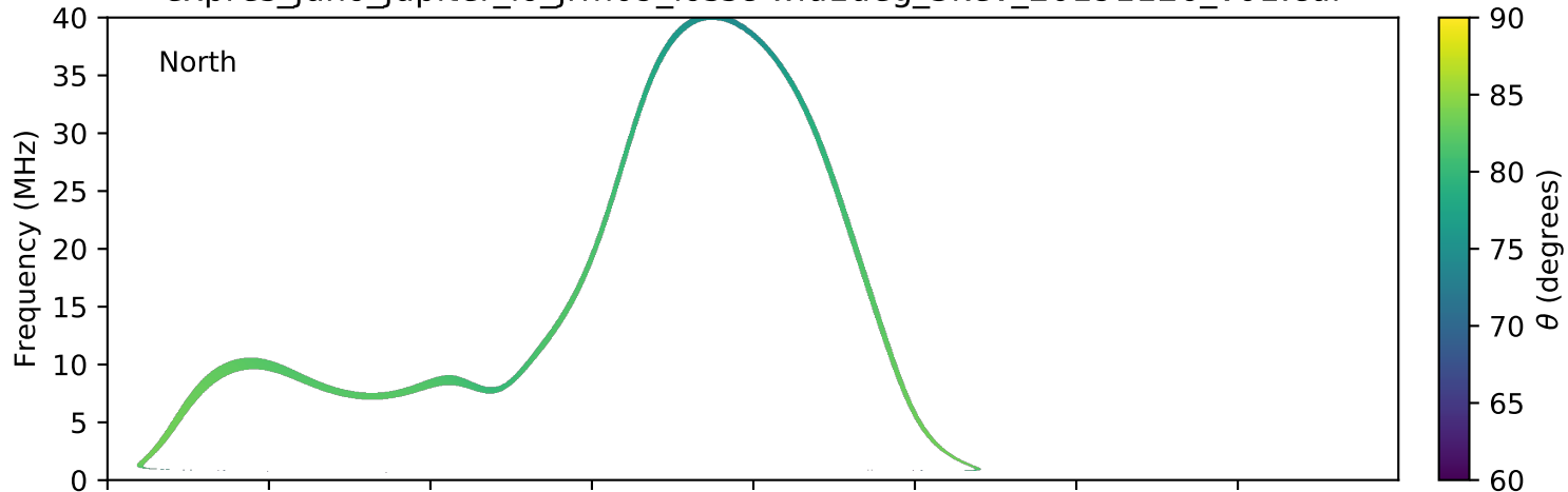
expres_juno_jupiter_io_jrm09_lossc-wid1deg_3kev_20191126_v01.cdf
