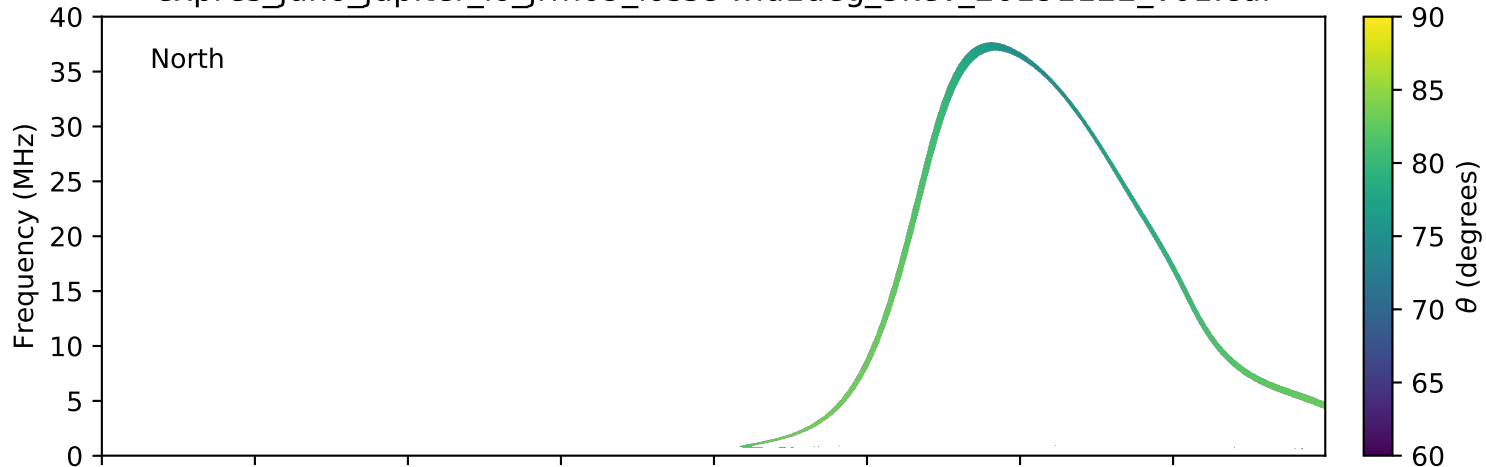
expres_juno_jupiter_io_jrm09_lossc-wid1deg_3kev_20191122_v01.cdf
