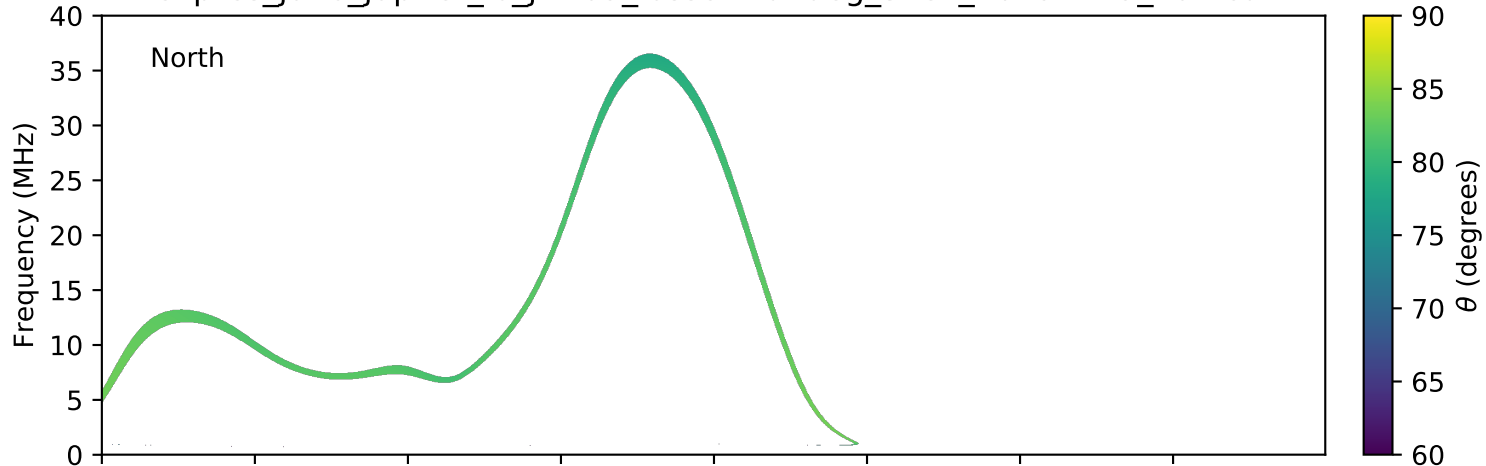
expres_juno_jupiter_io_jrm09_lossc-wid1deg_3kev_20191119_v01.cdf
