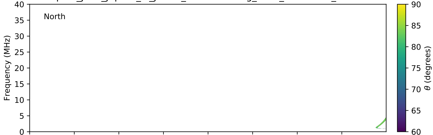
expres_juno_jupiter_io_jrm09_lossc-wid1deg_3kev_20191118_v01.cdf
