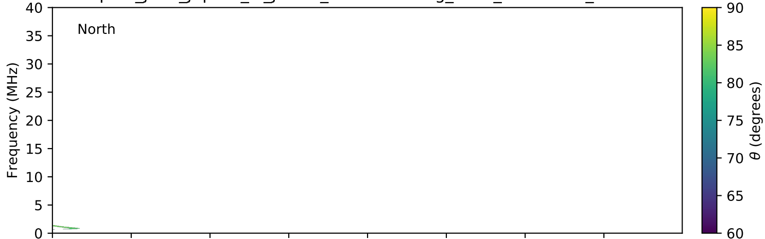
expres_juno_jupiter_io_jrm09_lossc-wid1deg_3kev_20191116_v01.cdf
