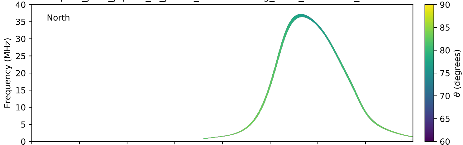
expres_juno_jupiter_io_jrm09_lossc-wid1deg_3kev_20191115_v01.cdf
