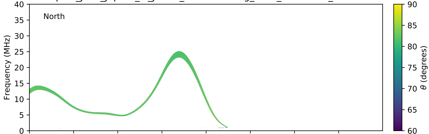
expres_juno_jupiter_io_jrm09_lossc-wid1deg_3kev_20191112_v01.cdf
