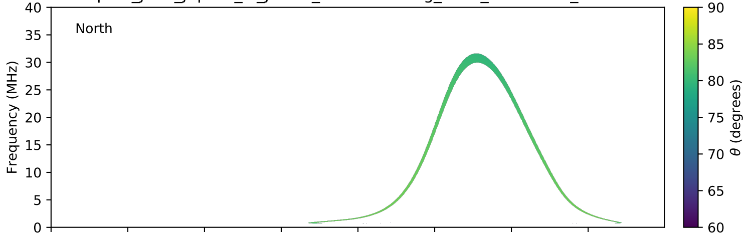
expres_juno_jupiter_io_jrm09_lossc-wid1deg_3kev_20191108_v01.cdf
