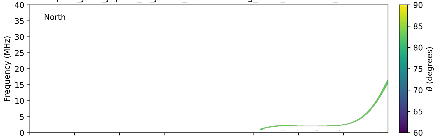
expres_juno_jupiter_io_jrm09_lossc-wid1deg_3kev_20191106_v01.cdf
