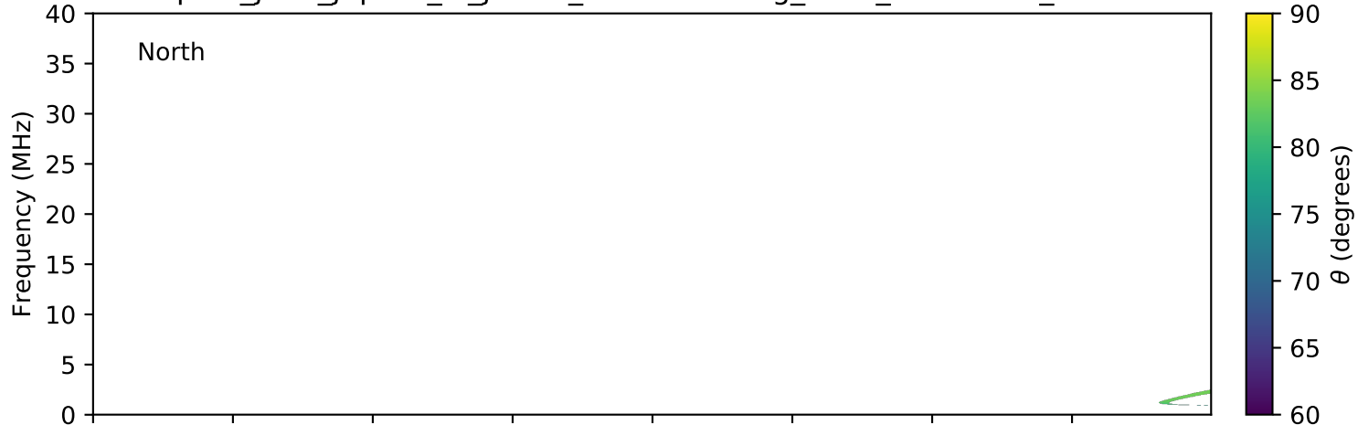
expres_juno_jupiter_io_jrm09_lossc-wid1deg_3kev_20191104_v01.cdf
