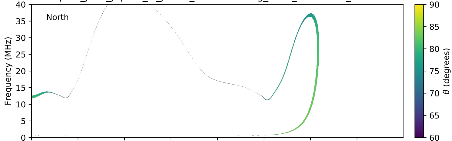
expres_juno_jupiter_io_jrm09_lossc-wid1deg_3kev_20191103_v01.cdf
