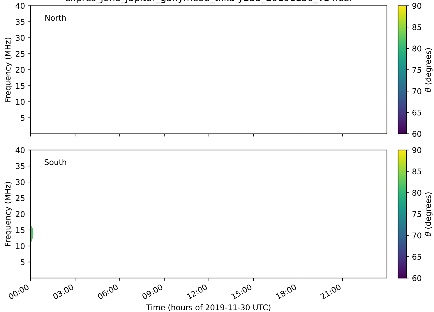
expres_juno_jupiter_ganymede_txka-y235_20191130_v14.cdf
