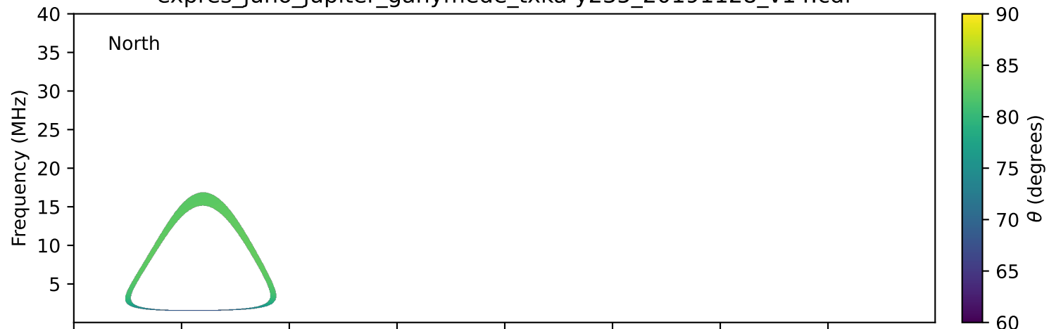
expres_juno_jupiter_ganymede_txka-y235_20191128_v14.cdf
