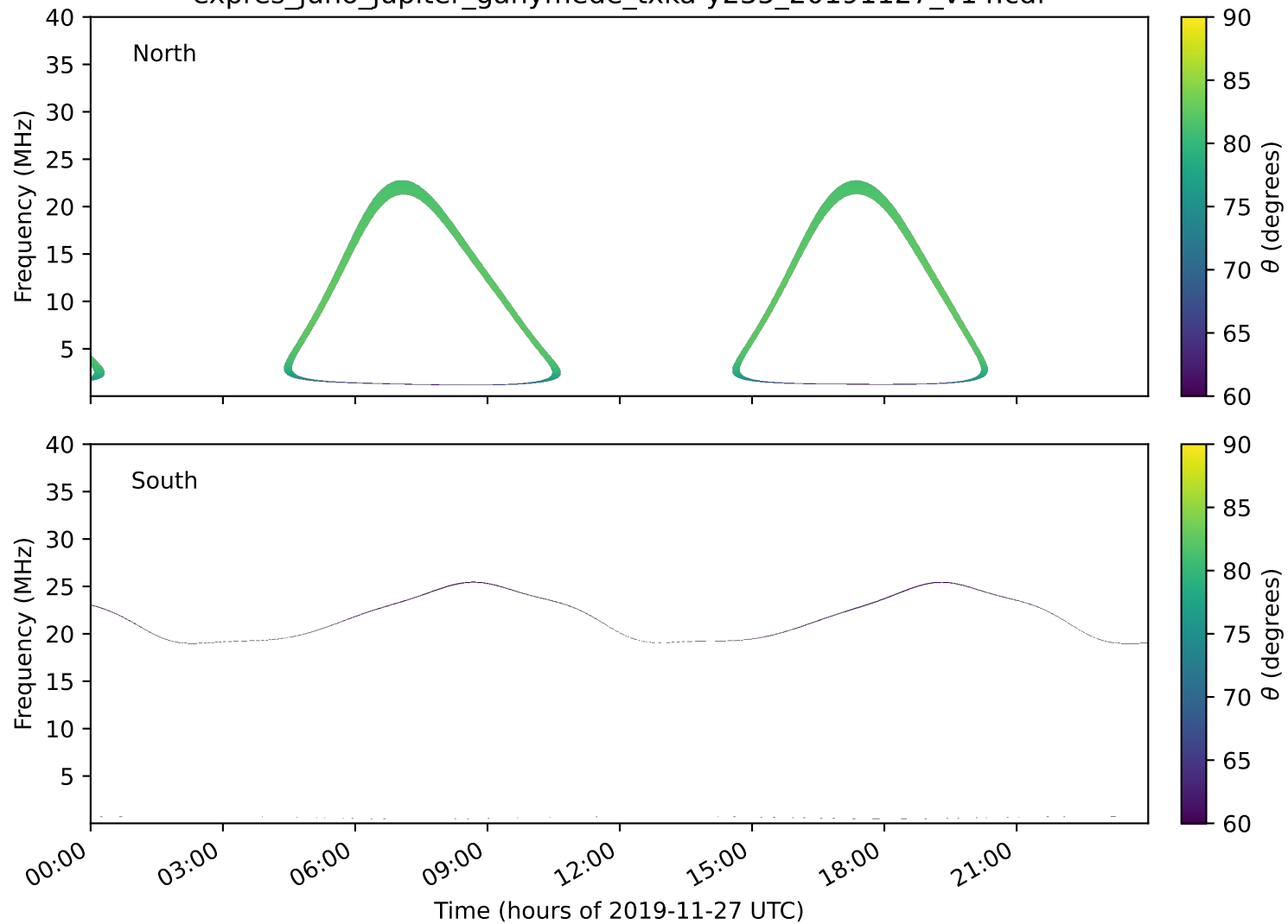
expres_juno_jupiter_ganymede_txka-y235_20191127_v14.cdf
