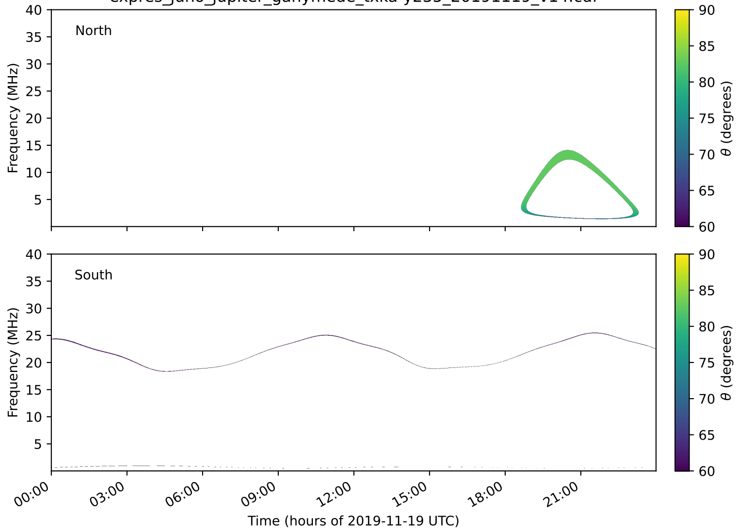
expres_juno_jupiter_ganymede_txka-y235_20191119_v14.cdf
