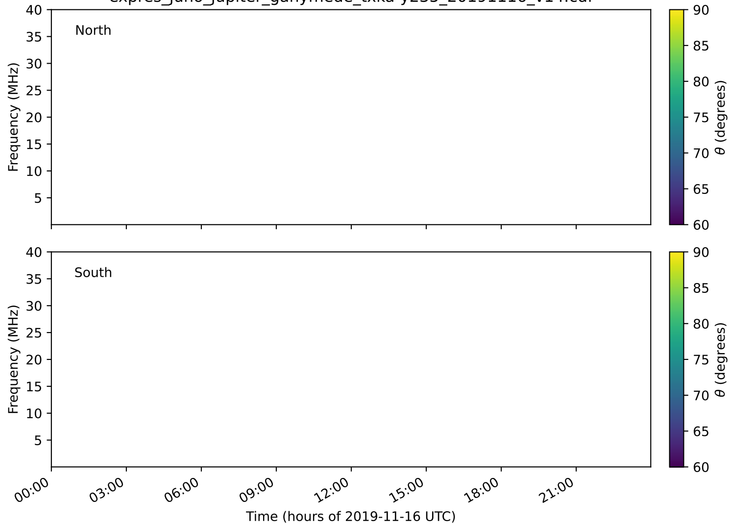
expres_juno_jupiter_ganymede_txka-y235_20191116_v14.cdf
