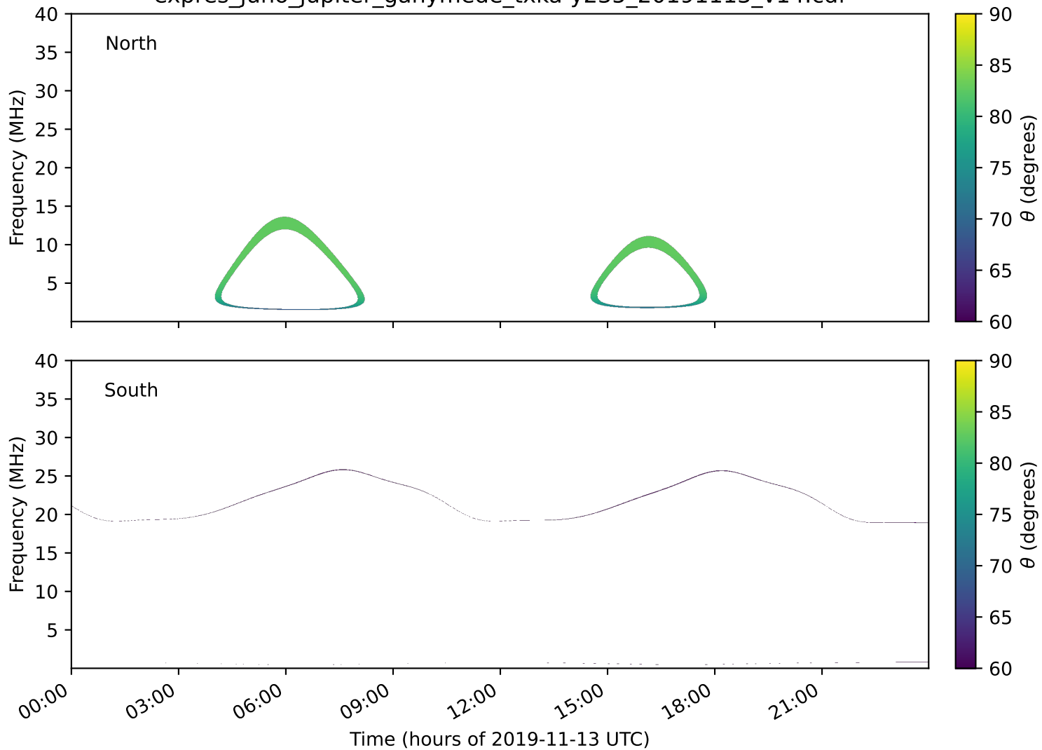
expres_juno_jupiter_ganymede_txka-y235_20191113_v14.cdf
