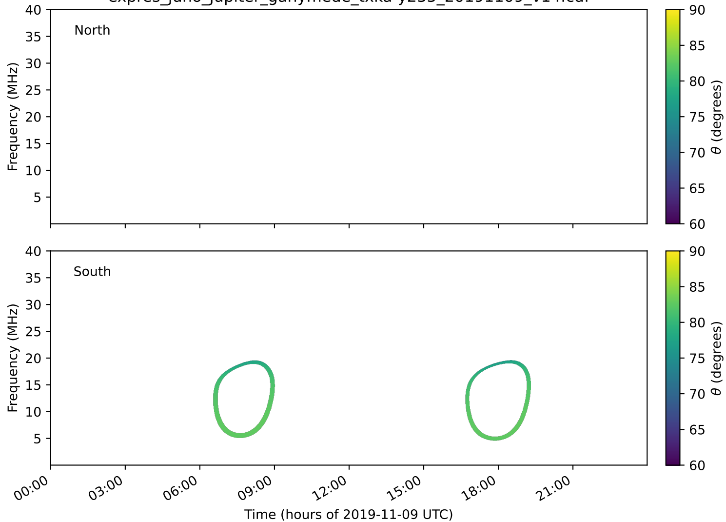
expres_juno_jupiter_ganymede_txka-y235_20191109_v14.cdf
