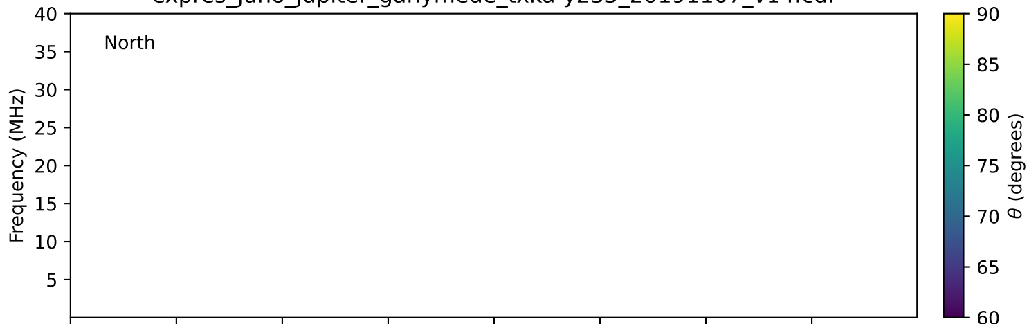
expres_juno_jupiter_ganymede_txka-y235_20191107_v14.cdf
