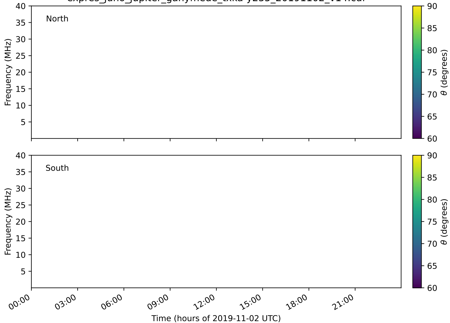
expres_juno_jupiter_ganymede_txka-y235_20191102_v14.cdf
